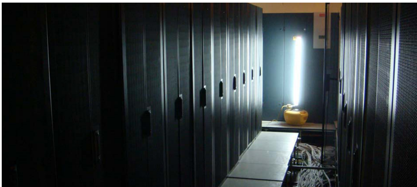
Tier 2 data centre with 48 server racks and ten comms racks plus an entrance facility housing another five comms racks
